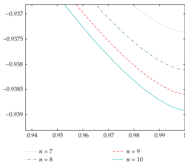
Figure 7: Numerical solutions of (5.43)-(5.1a) and a = 1 in the vicinity of t = 0 (a) and t = 1 (b). The step size is decreasing according to h = 1/2^n .
